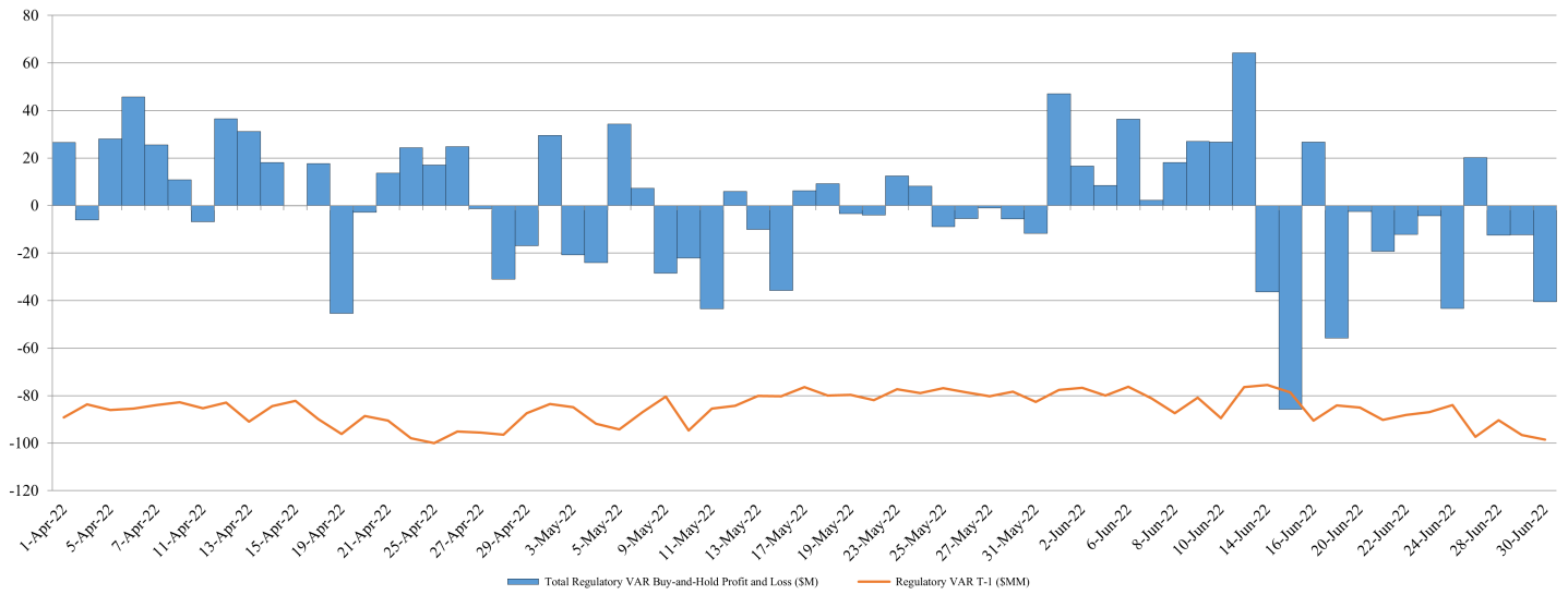
One-Day 99% Regulatory VAR and Associated Buy-and-Hold Profit and Loss ($M)
