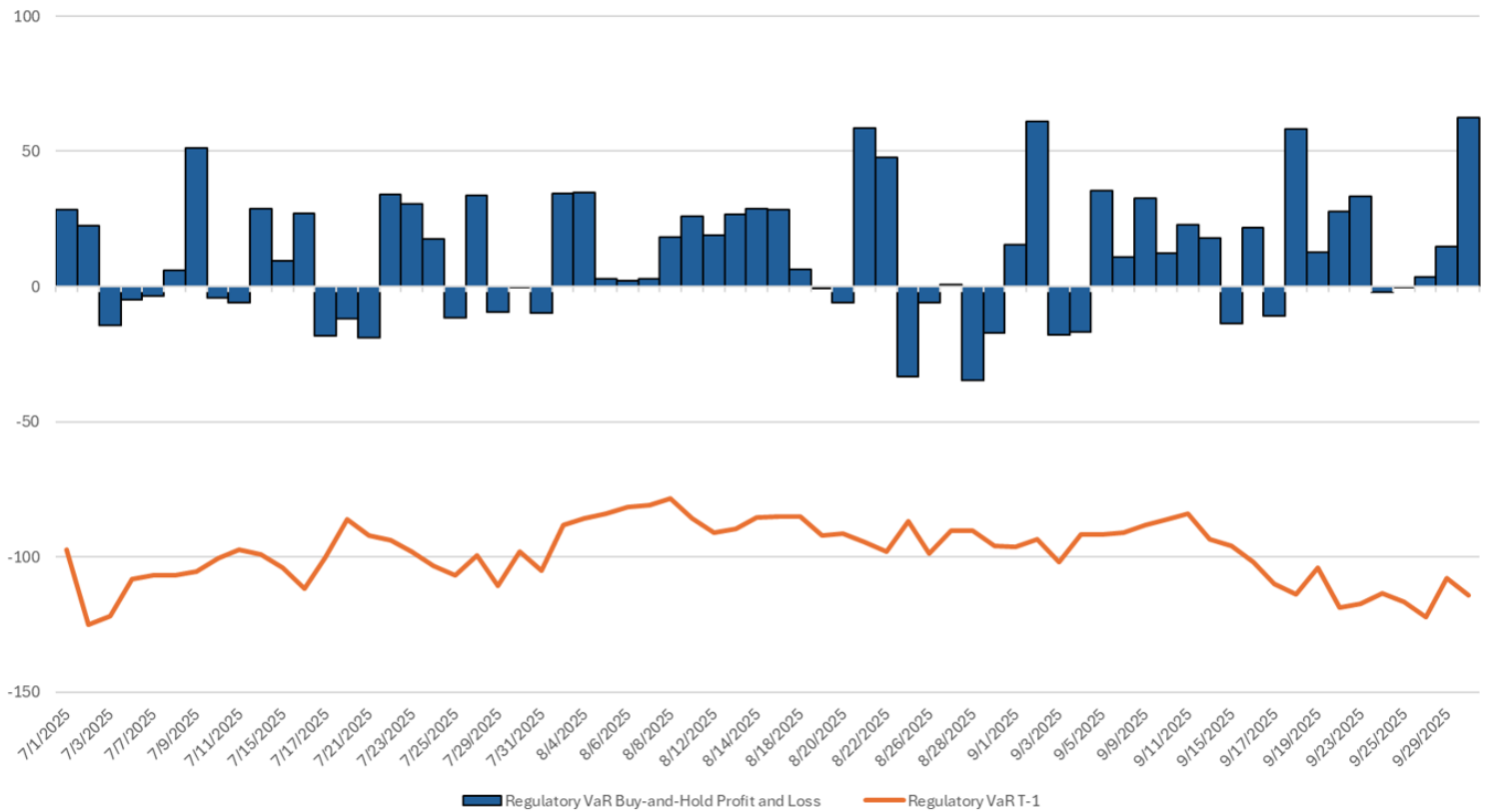
One-Day 99% Regulatory VaR and Associated Buy-and-Hold Profit and Loss ($M)
